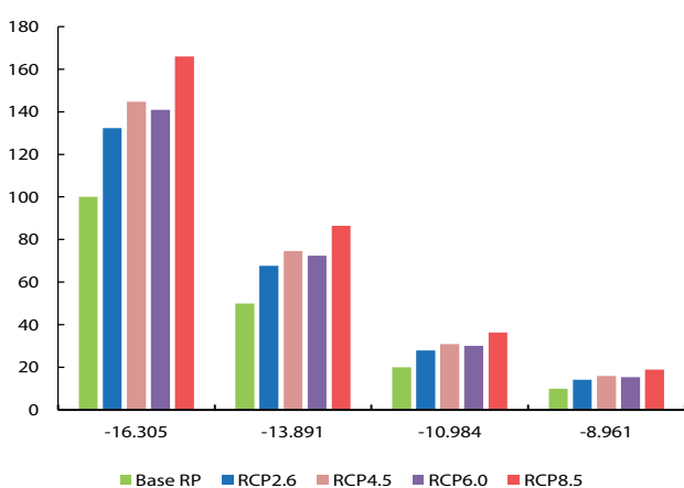
Figure A4.9 Change in return periods, 1 day with absolute min temperature (years), Shkoder
