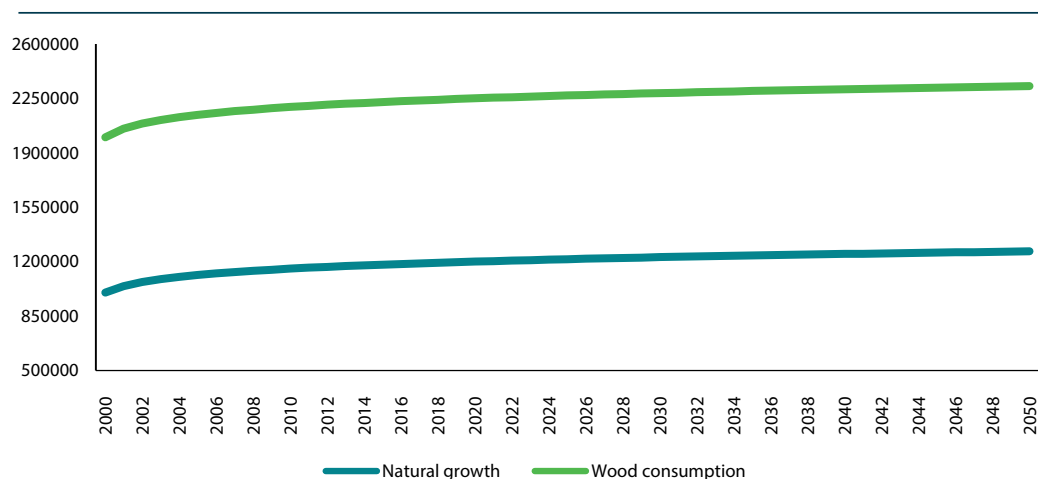
Figure 5.32 Projection of wood consumption and natural growth of forest (in m 3 ) for period 2000-2050
