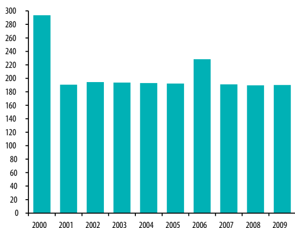
Figure 2.14 Fuel wood consumption (kTOE) for energy purposes (2000 - 2009)
