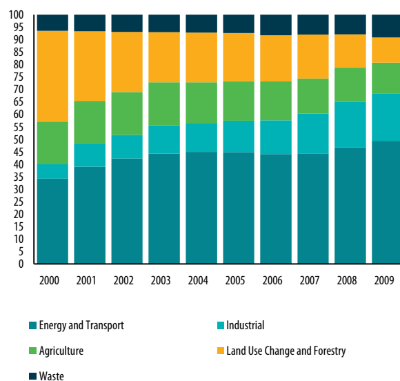
Figure 2.2 CO 2 eq. emissions from all economic sectors (2000 - 2009) (%)
