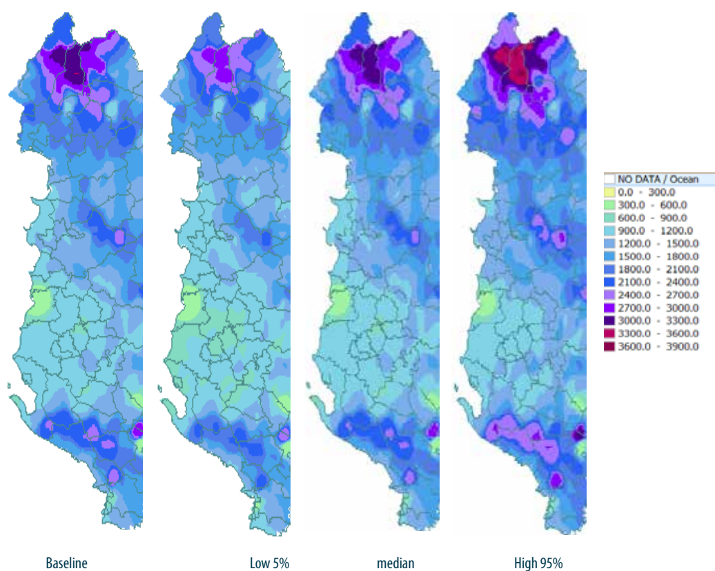
Figure A4.11 Precipitation distribution, baseline and expected changes by 2050 (average and 5% and 95% levels)
