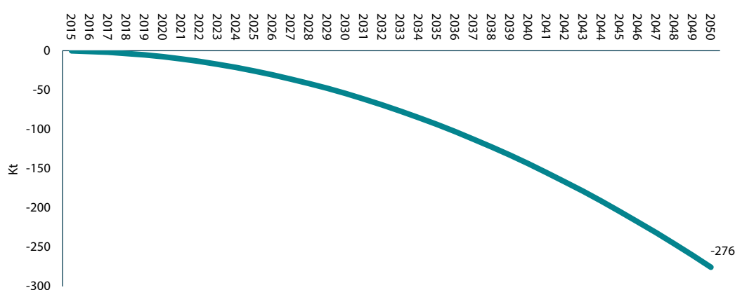
Figure 5.26 Potential CO 2 sequestration by adopting agro-forestry practices 2015-2050 (in Gg)
