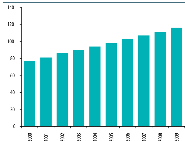
Figure 2.32 CO 2 eq. emissions from Chemical Industry, 2000 - 2009 (Gg)
