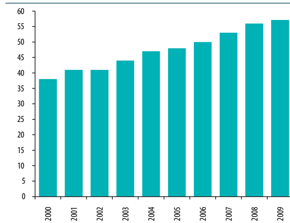
Figure 2.31 CO 2 eq. emissions from Cement Production, 2000-2009 (Gg)
