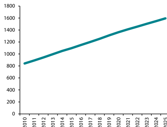
Figure 5.41 Waste sector projections of CO 2 eq. emissions (in Gg)
