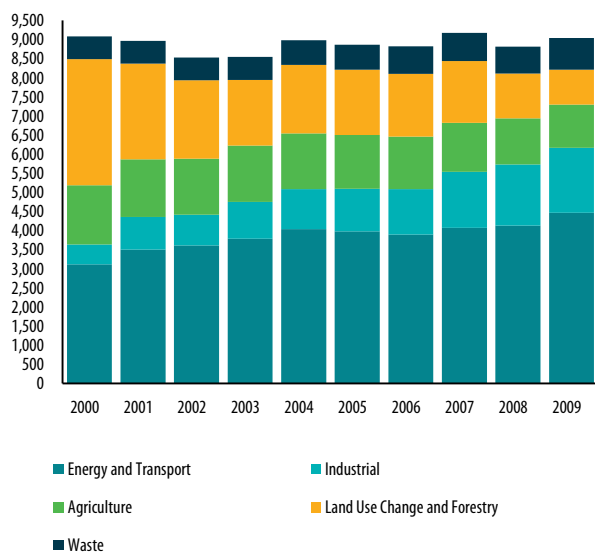
Figure 2.1 CO 2 eq. emissions from all economic sectors (2000 - 2009) (Gg)
