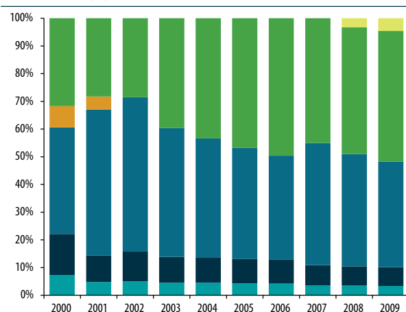
Figure 2.35 CO 2 eq. emissions from Industrial sub-sectors, 2000 - 2009 (%)
