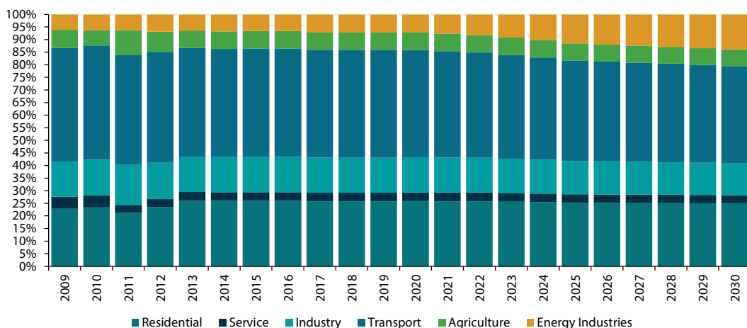
Figure 5.19 Share of GHG emissions by sectors (in %)
