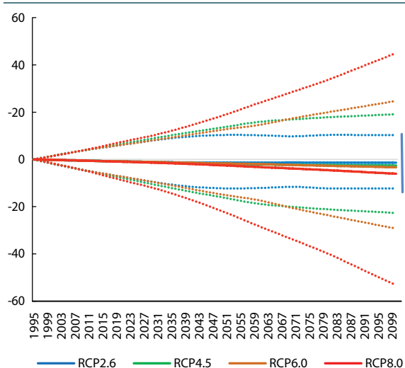
Figure A4.12 Changes and variability of annual precipitation (%), different scenarios. Median estimates are given as full lines and the lower and upper bound given as dotted line. (Lezhe)
