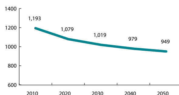
Figure 5.28 Baseline scenario of GHGs emissions from livestock in Gg of CO 2 eq., for the period 2020-2050
