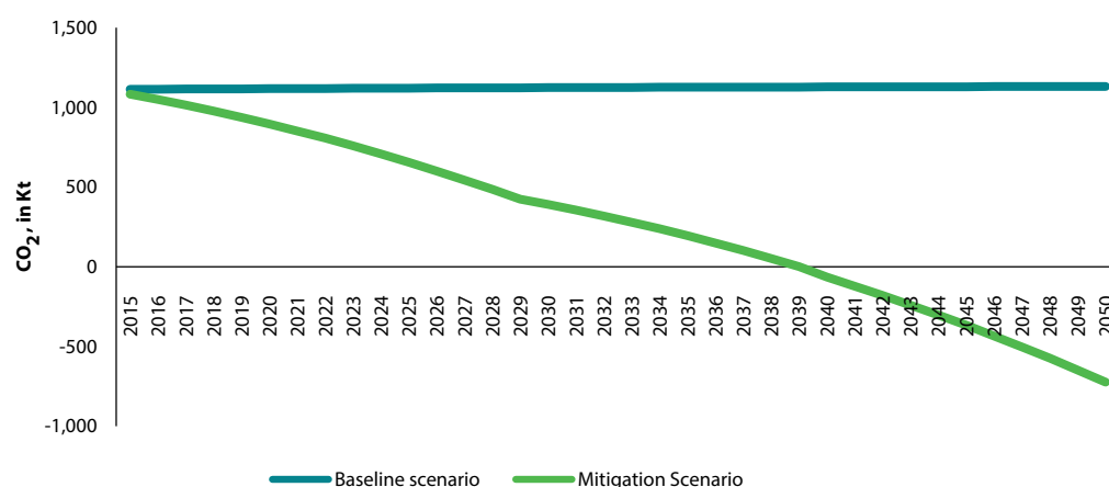
Figure 19 CO 2 balance for period 2015-2050 (in Gg), under the Baseline and Mitigation Scenario (TI+AFF 1,000 ha/yr)
