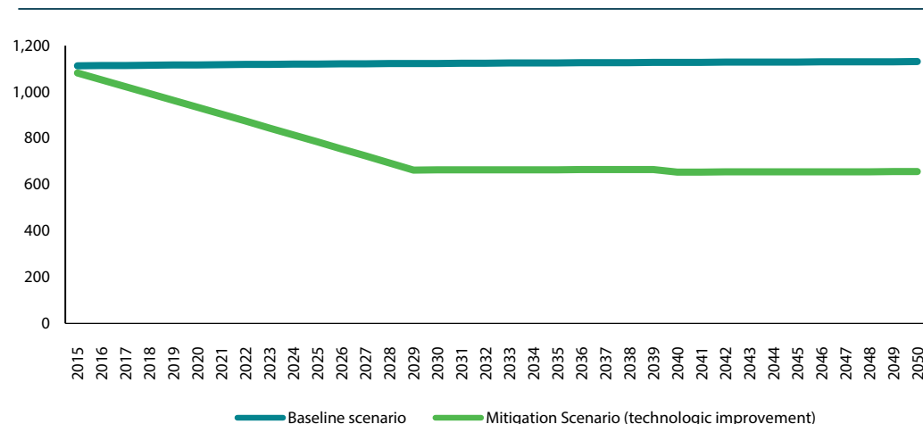
Figure 5.33 Projected CO 2 emissions from forests (in Gg), during the period 2015-2050
