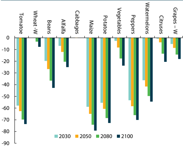
Figure 4.23 Crop yield reduction (%) under scenario “without irrigation”
