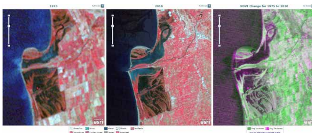
Figure 4.20: Actual change of the coastline, Kune-Vaini lagoons, (lilac-loss of vegetation, green-vegetation increase).
