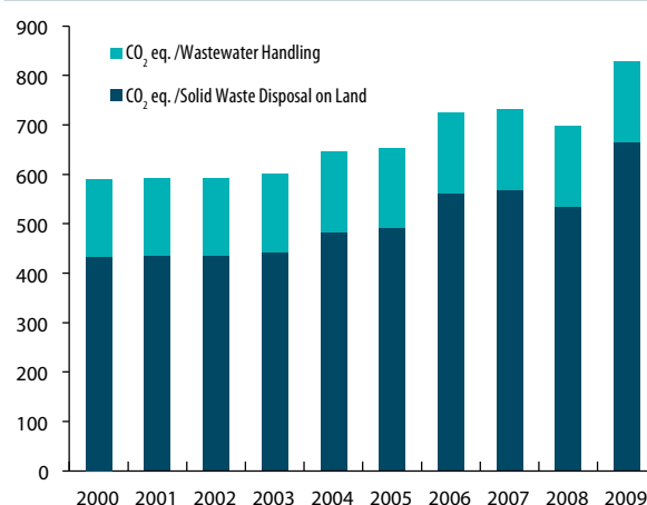
Figure 2.39 CO 2 eq. emissions from Waste subsectors, 2000 - 2009 (Gg)
