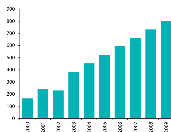
Figure 2.33 CO 2 eq. emissions from Metal Production, 2000 - 2009 (Gg)
