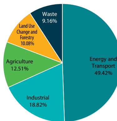
Figure 2.4 CO 2 eq. emissions from all economic sectors for the year 2009 (%)
