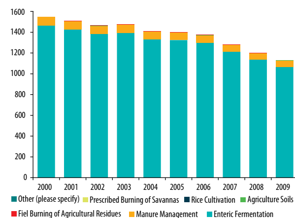
Figure 2.27 Total emissions in CO 2 eqv. from Agriculture sub-sectors, 2000 - 2009 (Gg)
