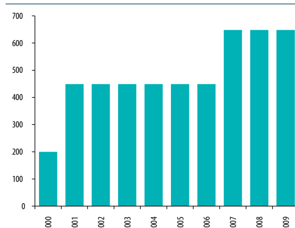
Figure 2.33 CO 2 eq. emissions from Metal Production, 2000 - 2009 (Gg)
