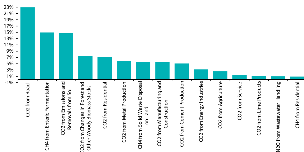
Figure 2.41 GHG Key Sources for the year 2005
