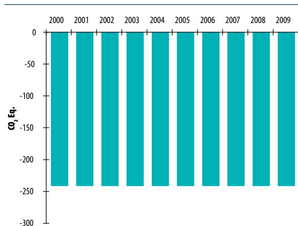
Figure 2.19 Emissions from abandonment of managed lands (Gg)
