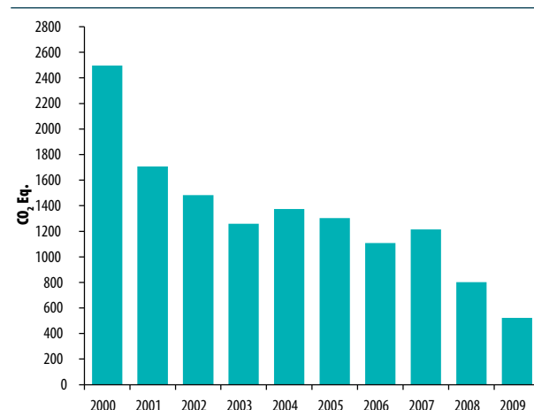
Figure 2.20 Emissions from changes in soil carbon for mineral soil (Gg)
