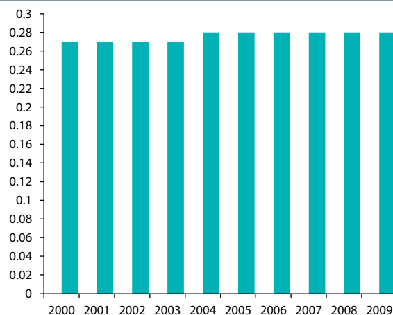
Figure 2.37 N 2 O emissions from Wastewater handling subsector, 2000 - 2009 (Gg)
